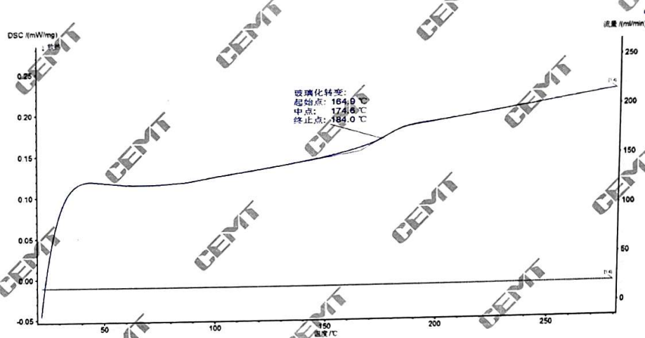
图10 玻璃化转变温度曲线 Fig.10 Glass transition temperature curve
