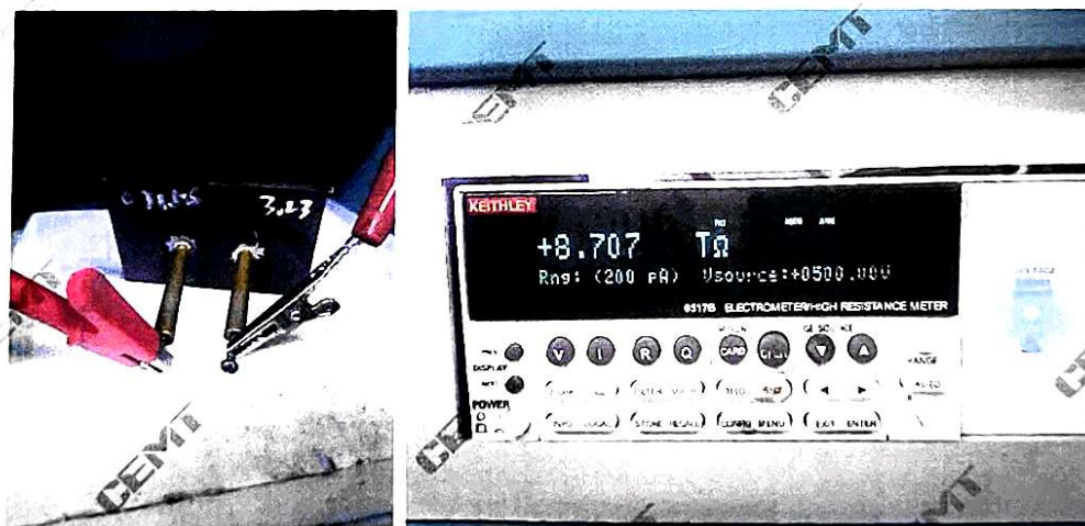
图7 绝缘电阻试验 Fig.7 Insulation resistance test
