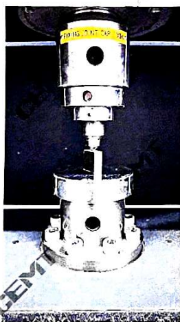
图9 粘合强度试验 Fig.9 Adhesion strength test
