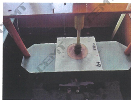
图4 垂直层向电气强度试验 Fig.4 Electric strength perpendicular to laminations test
