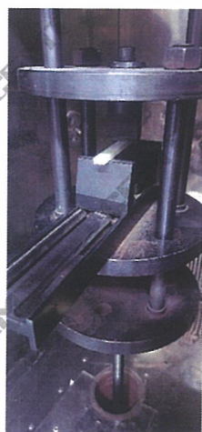
Fig.1 Flexural strength perpendicular to laminations test
